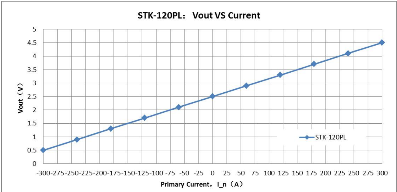
The dependence of Vout of STK-120PL on the primary current.
