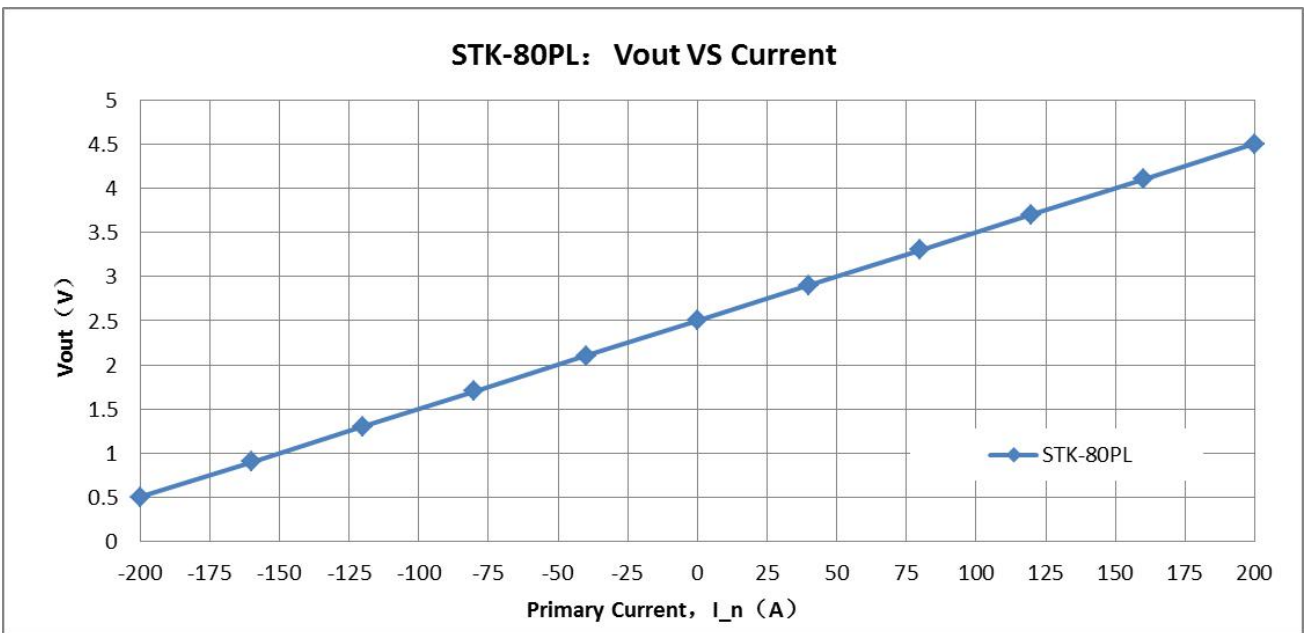
The dependence of Vout of STK-80PL on the primary current.
